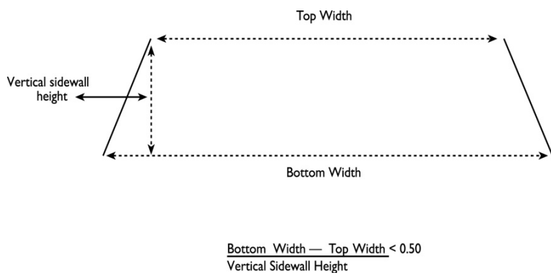
Diagram 15 Cross Section of Unstrung Head
